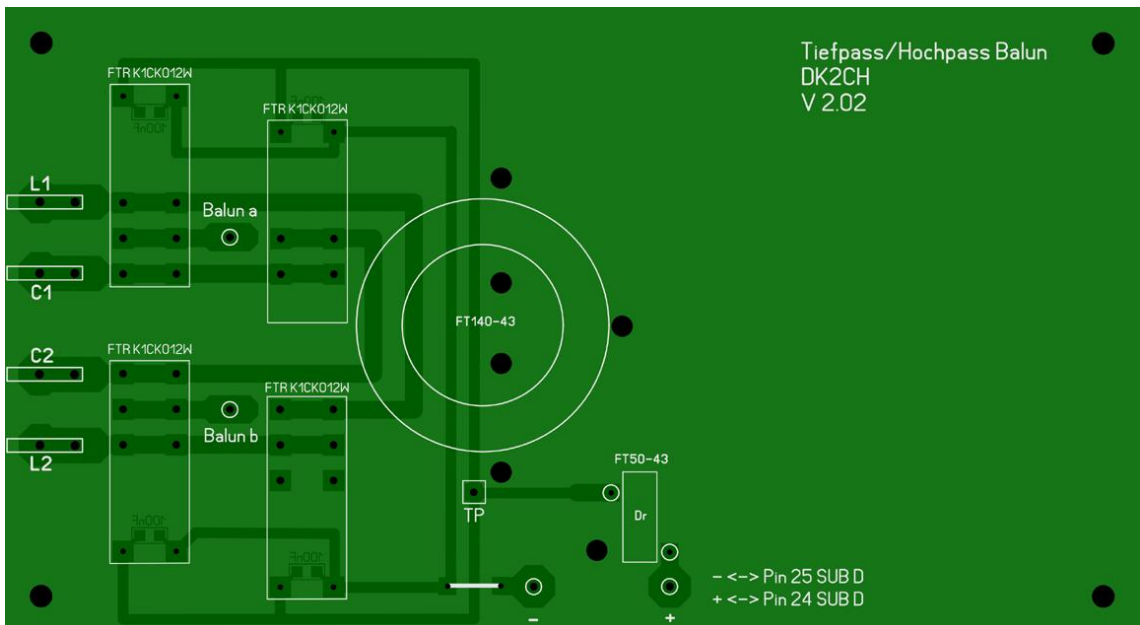
DK2CH-Balun-V2.02-TOP
