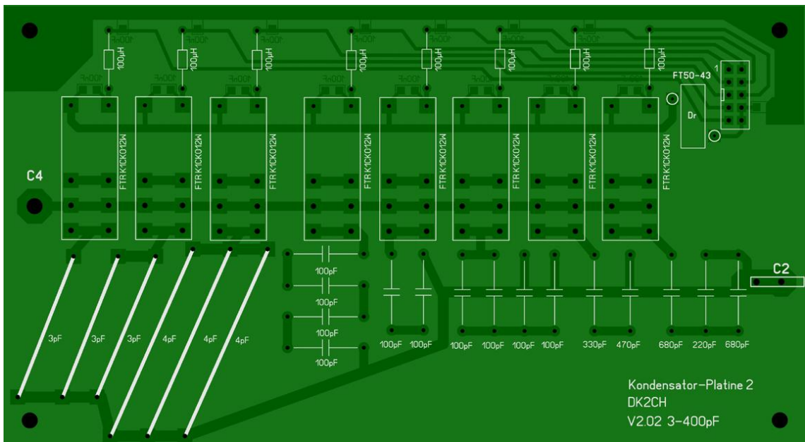
DK2CH-C-Bank2-V2.02-TOP
