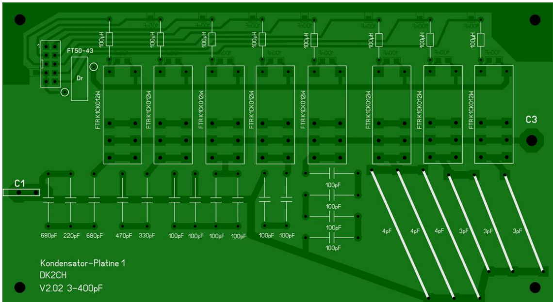
DK2CH-C-Bank1-V2.02-TOP
