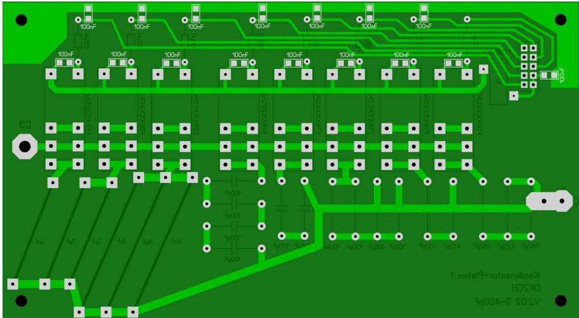
DK2CH-C-Bank1-V2.02-BOT
