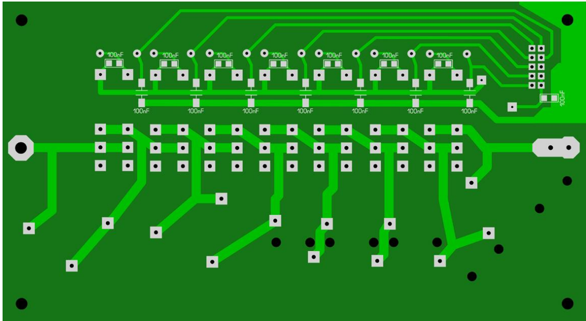
DK2CH-Spulen-Platine-1-BOT
