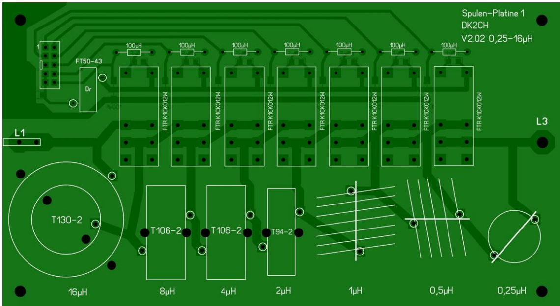
DK2CH-Spulen-Platine-1-TOP
