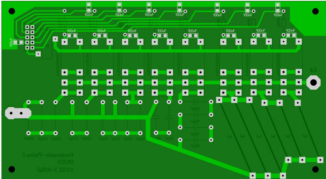
DK2CH-C-Bank2-V2.02-BOT
